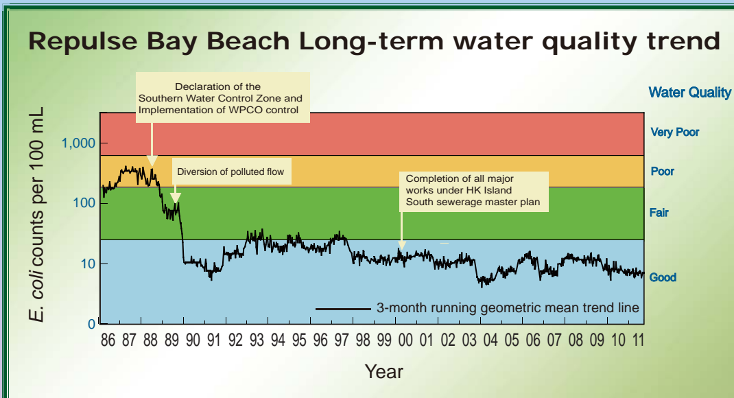
Improvement work to divert away polluted storm flow and improve beach environment
